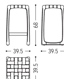
BUNGALOW BS-68
