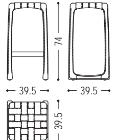
BUNGALOW BS-74
